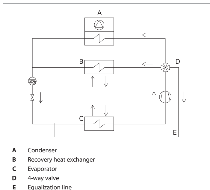
Refrigerant circuit
